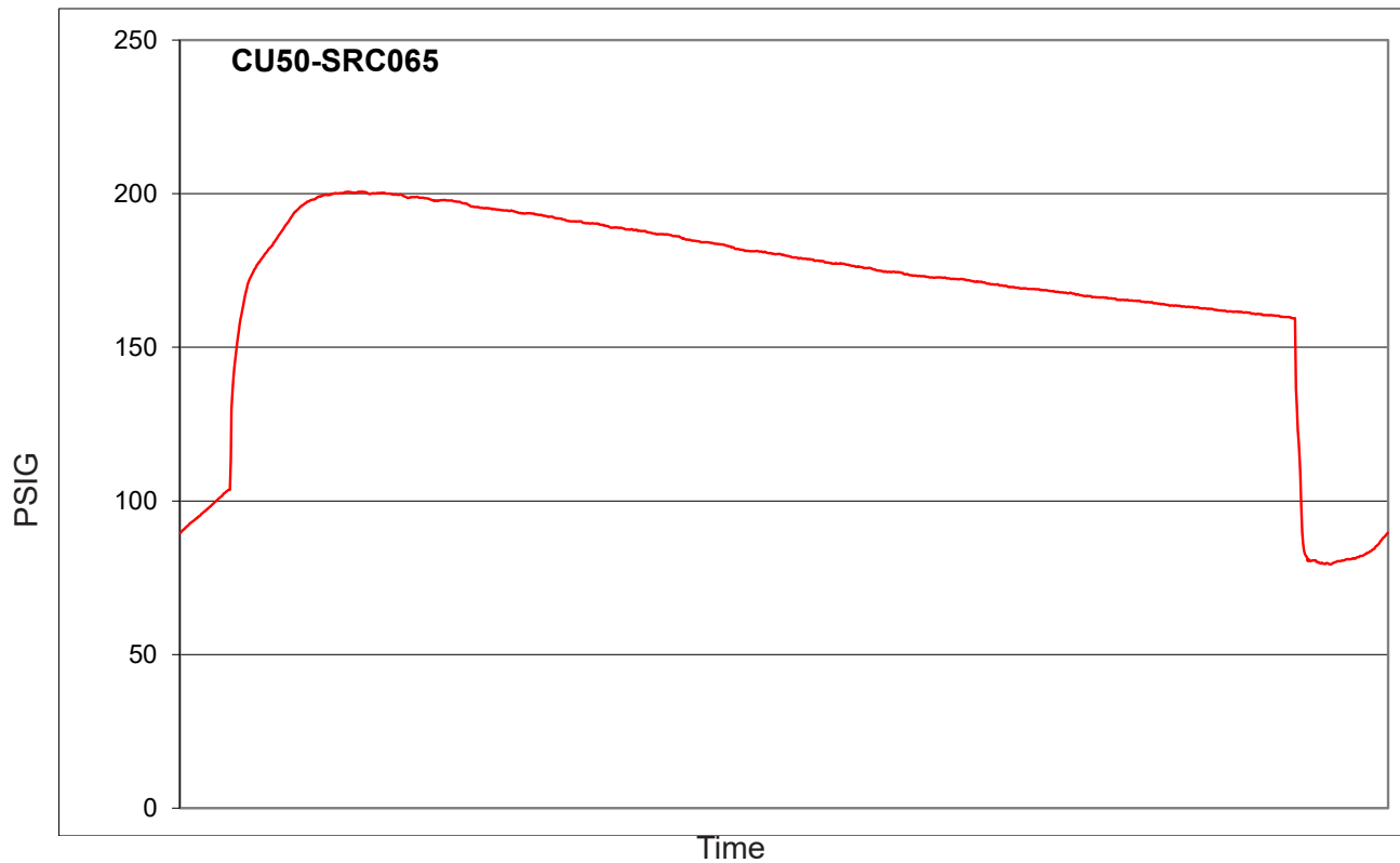
Discharge Pressure
